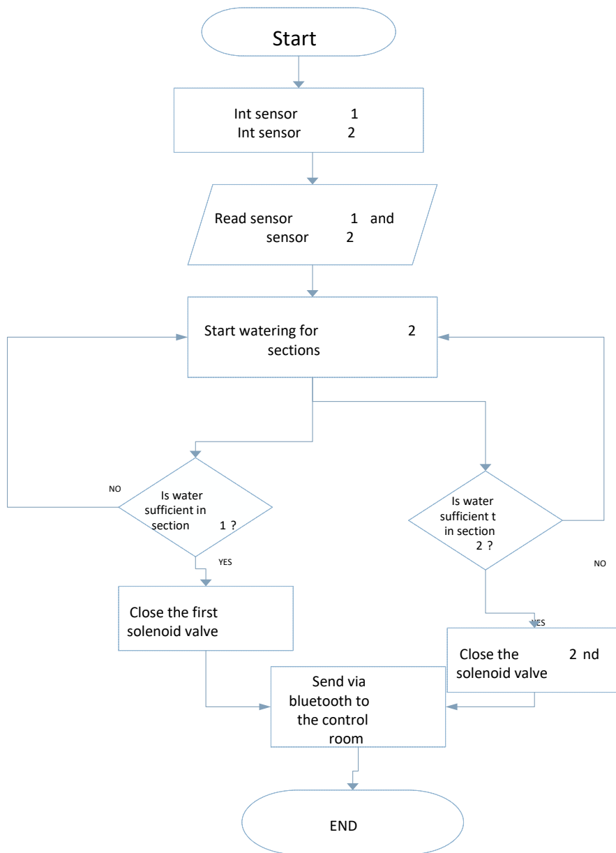
Figure 7. Flowchart of the system
