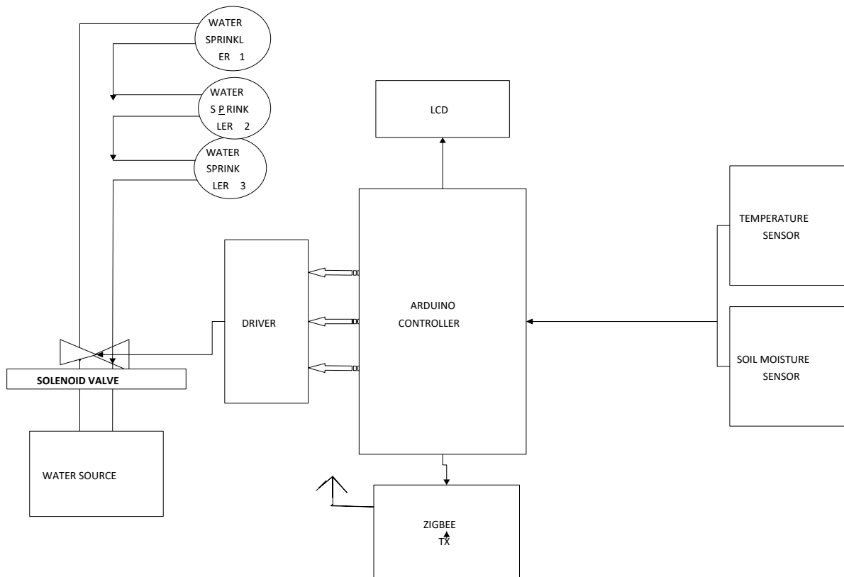
Figure 1. Block Diagram of the System Transmitter
