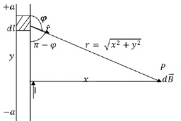
Fig 1: A section of a Straight Current Carrying Conductor Applying the Biot-Savart law, we find the magnitude of the field
