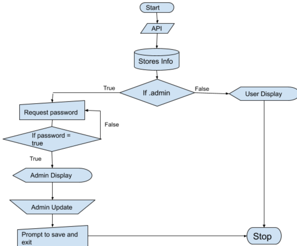
Control Flowchart of the above Algorithm
