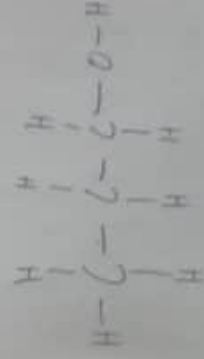
Propan-1-ol
