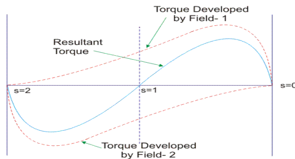
Torque Slip Characteristics of Single Phase Induction Motor
